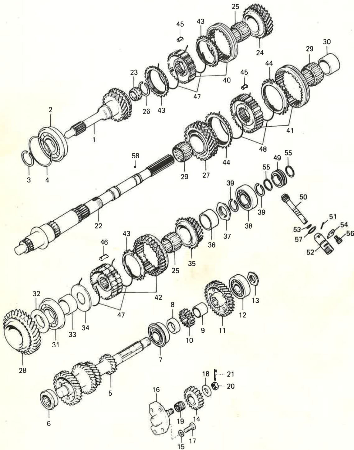
TRANSMISSION GEARS - 5 SPEED
