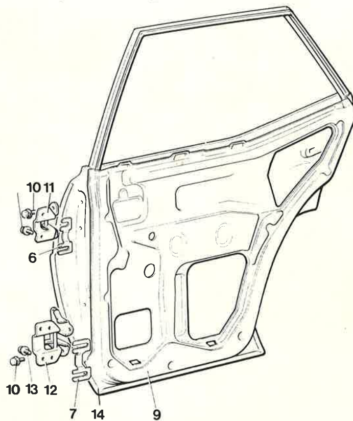
DOORS AND HINGES
