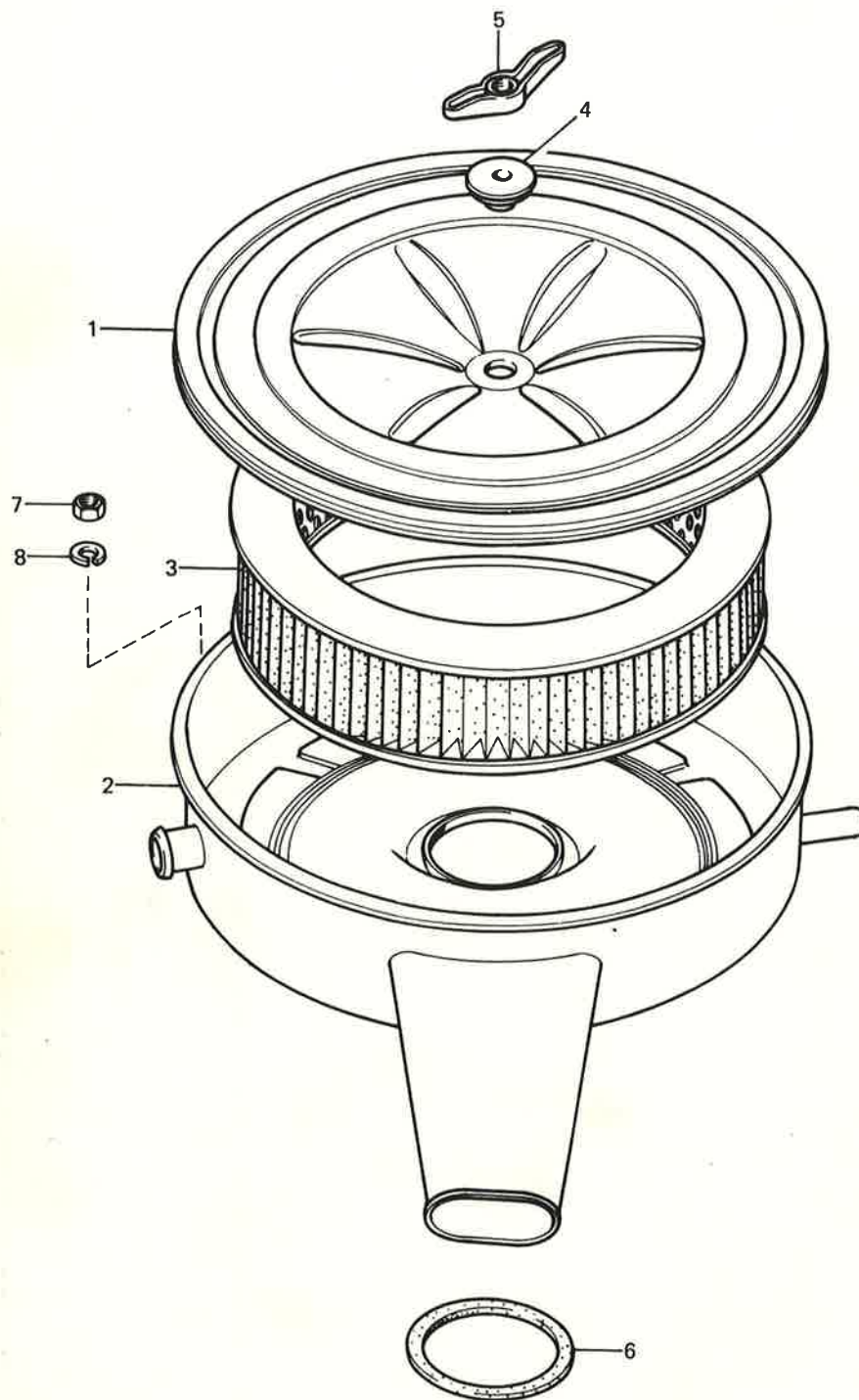
AIR CLEANER SATURN ENGINE
