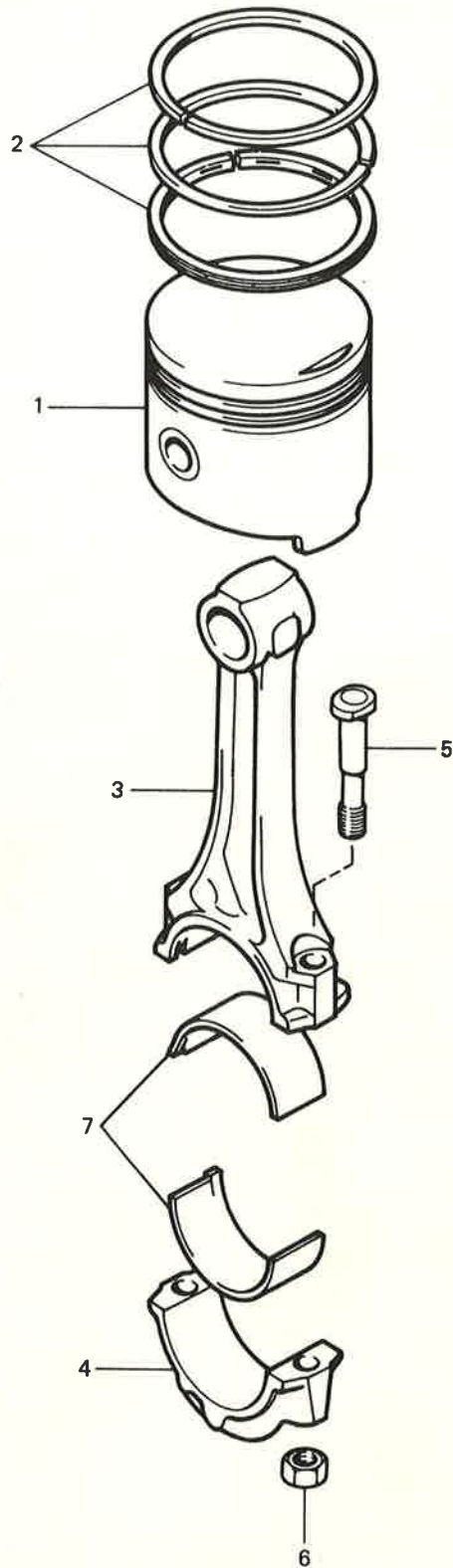
PISTON & CONNECTING ROD
