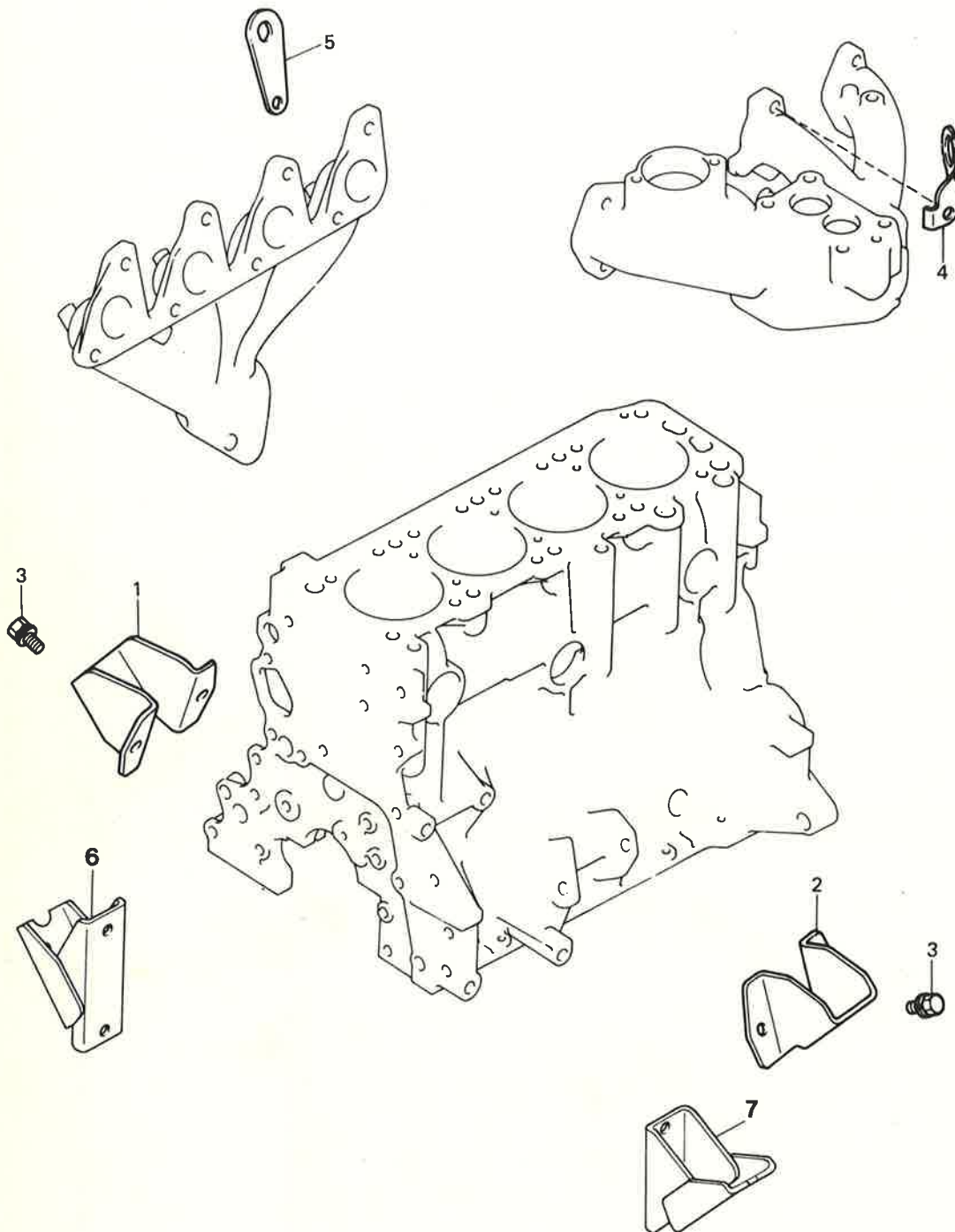
ENGINE SUPPORTS
