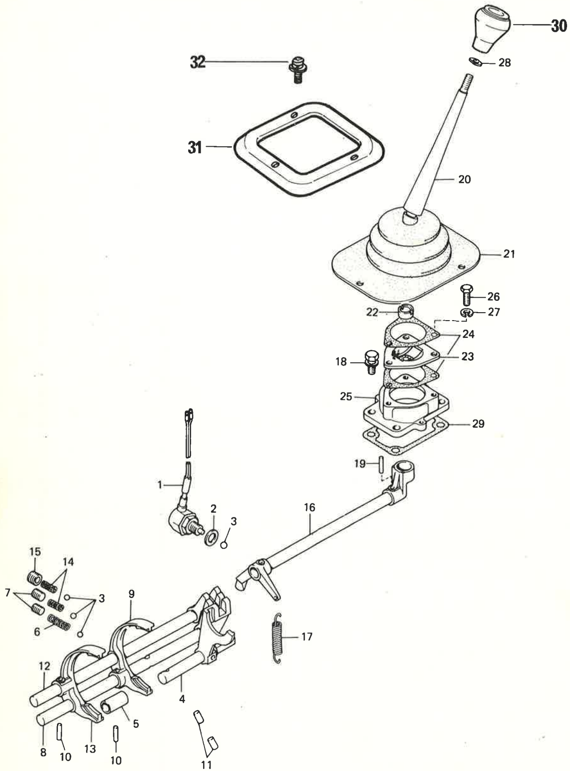
TRANSMISSION SHIFT 4 SPEED
