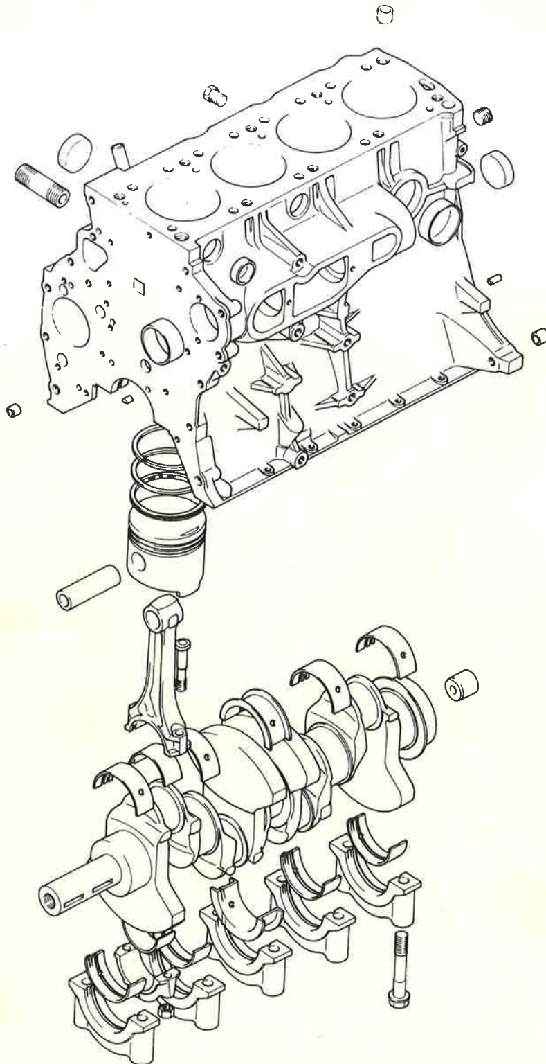
SHORT ENGINE
