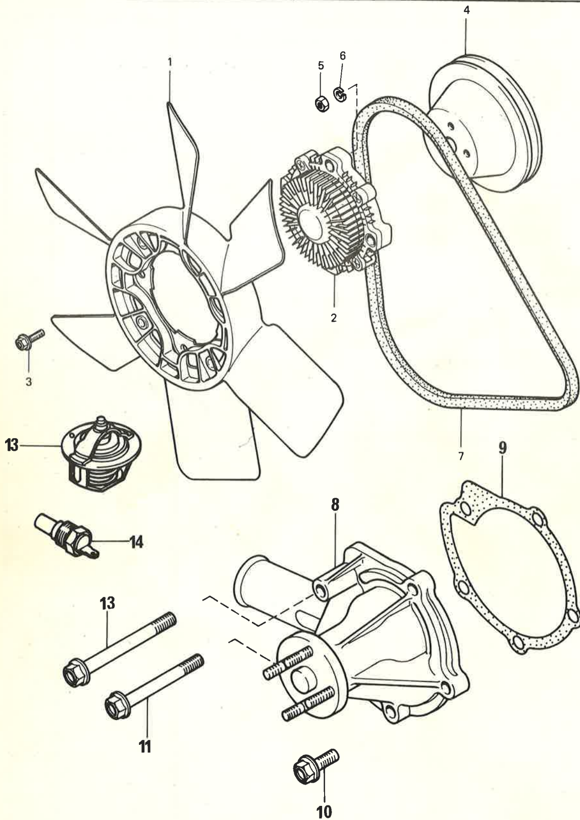
FAN, PUMP AND BELT - ASTRON ENGINE
