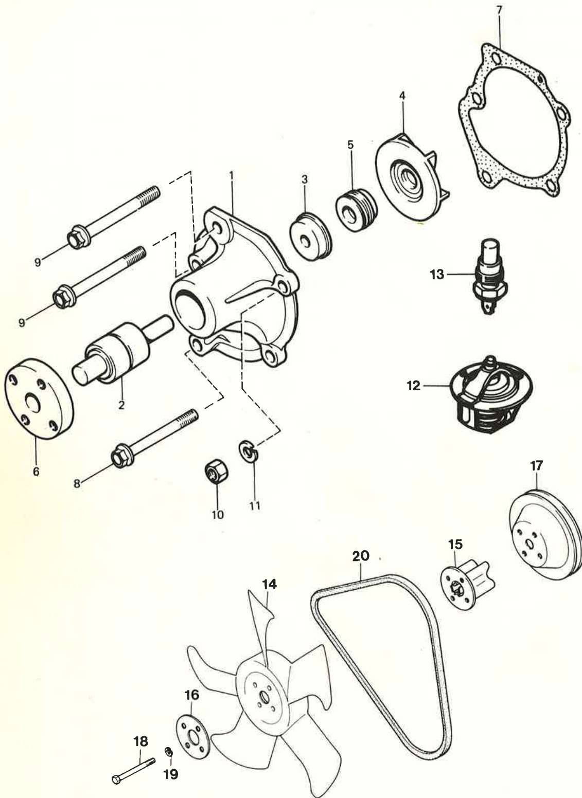
FAN , PUMP AND BELT SATURN ENGINE
