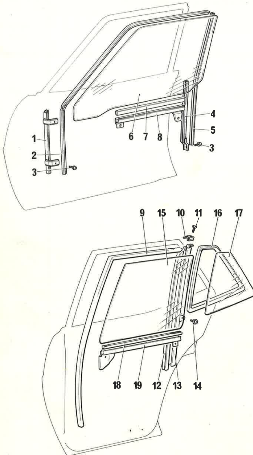
DOOR WINDOW AND SASH
