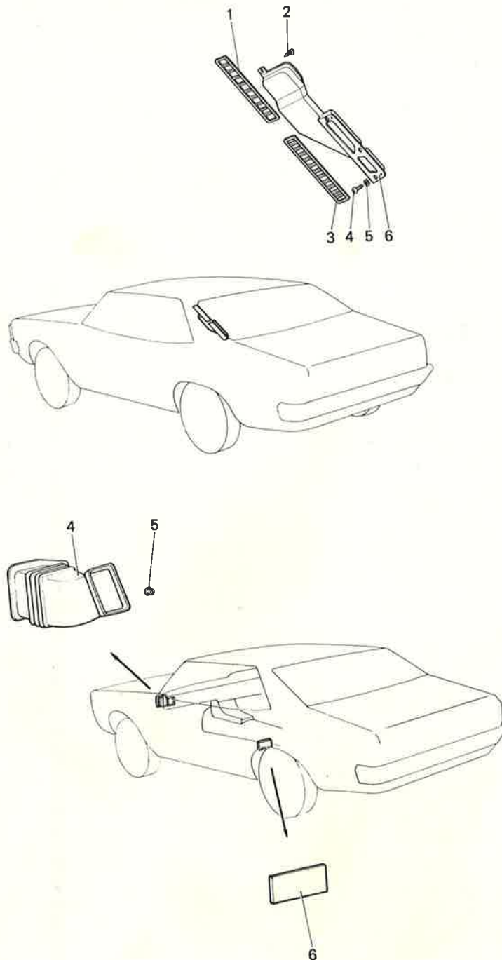
REAR VENTILATION AND SIDE DUCT
