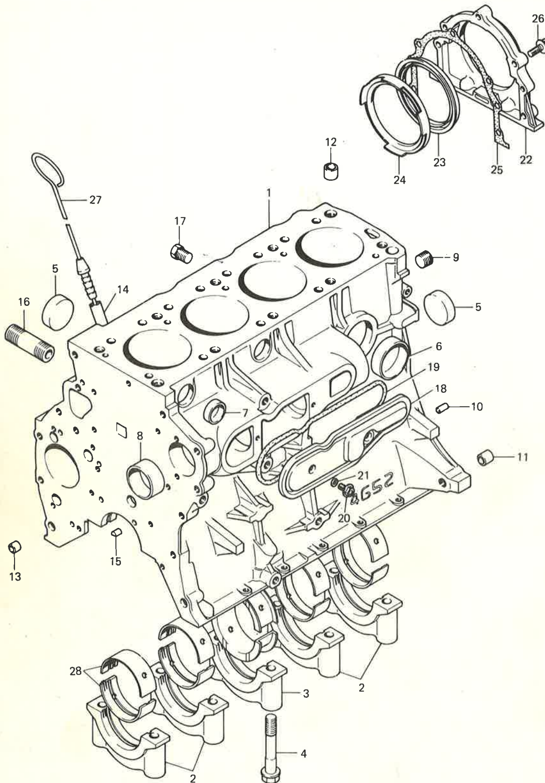
CYLINDER BLOCK - ASTRON ENGINE
