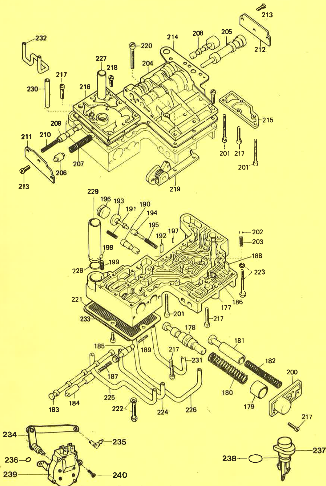
VALVE GEAR, INHIBITOR SWITCH & BREATHER
