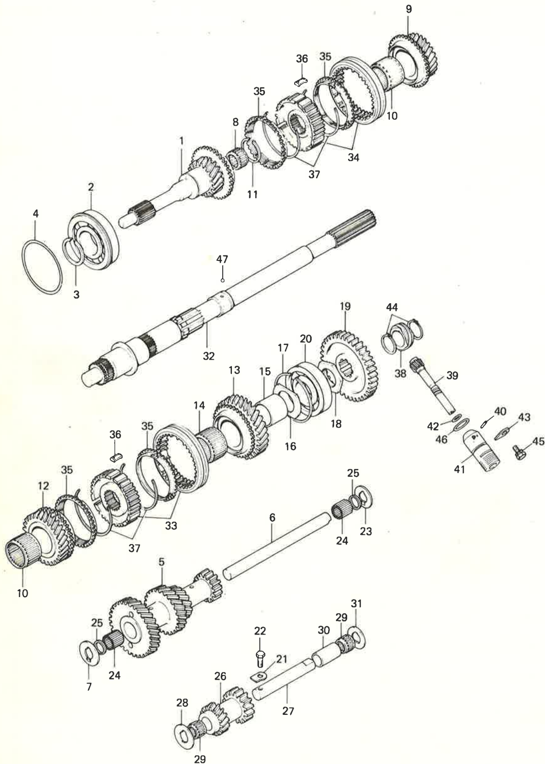
TRANSMISSION GEARS 4 SPEED
