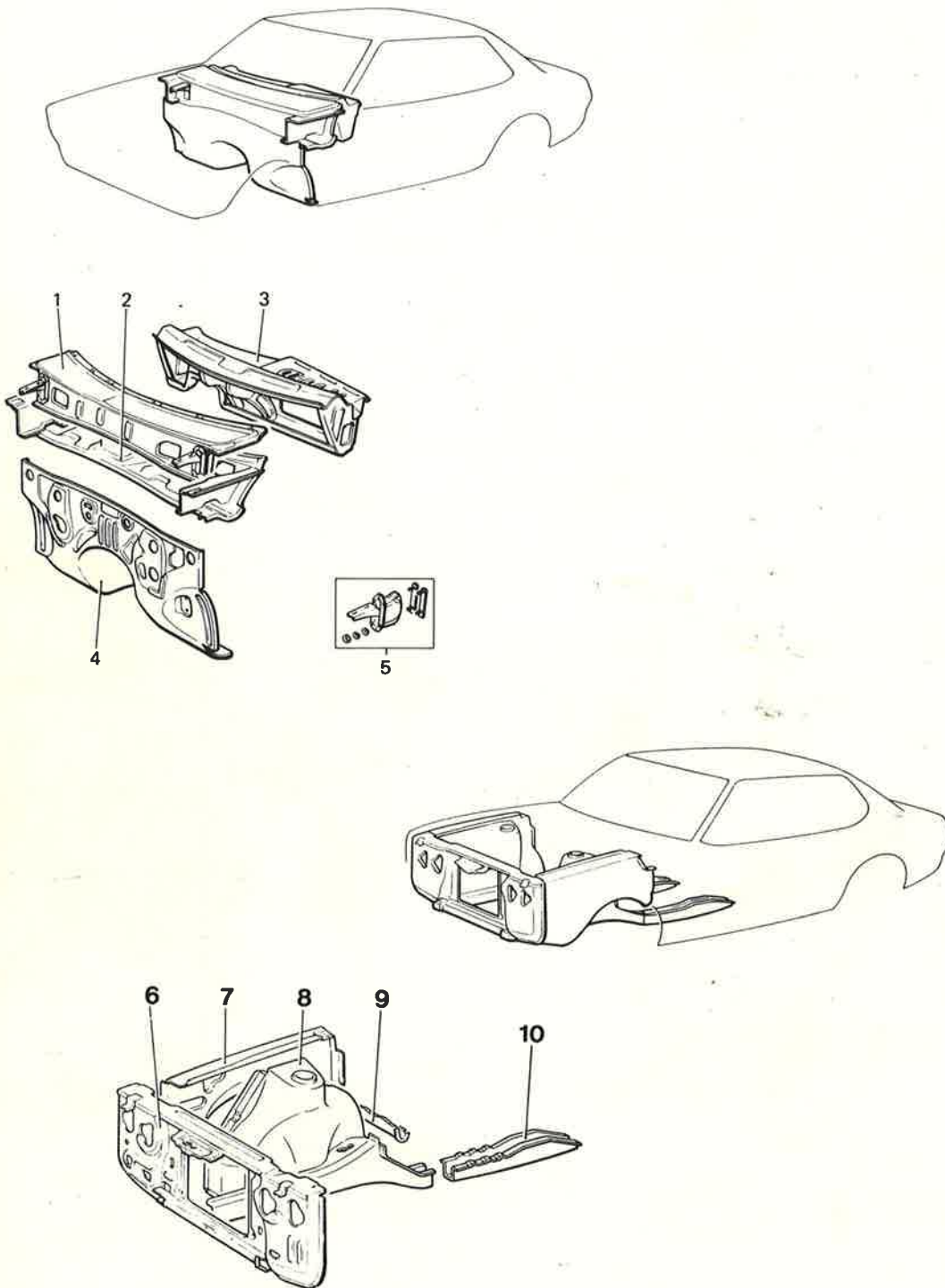
FRONT PANELS
