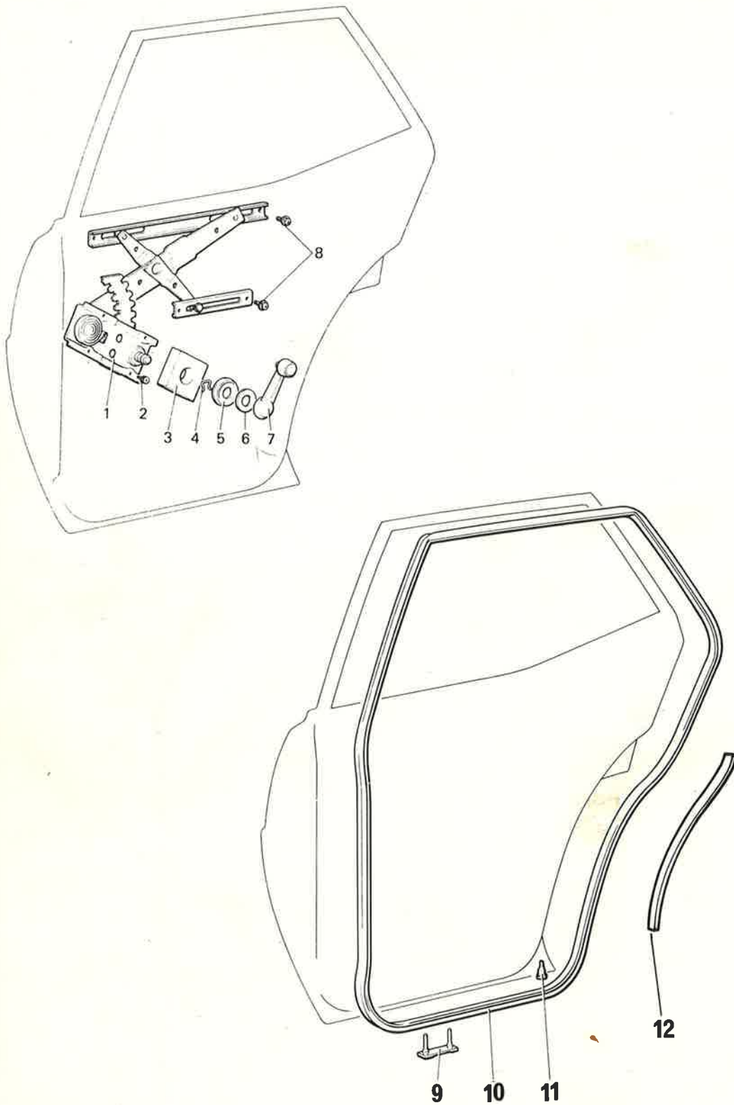
REAR DOOR REGULATOR AND WEATHERSTRIP
